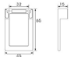
Model: SYJ0155 Material: Zinc Chrome Plated
