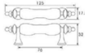
Model: SYJ0245 Material: Zinc & Ceramic Antique Bronze
