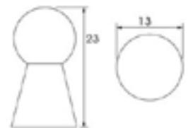
Model: SYJ3479 Material: Zinc Chrome Plated
