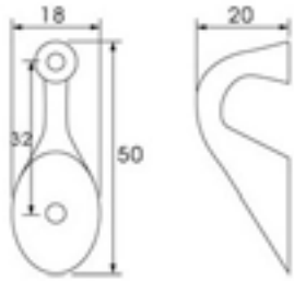
Model: SYJ3305 Material: Zinc Chrome Plated
