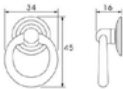
Model: SYJ3430 Material: Zinc Chrome Plated
