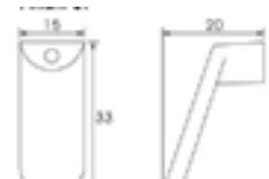
Model: SYJ3304 Material: Zinc Chrome Plated
