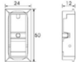
Model: SYJ3249 Material: Zinc Chrome Plated
