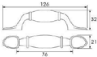
Model: SYJ0246 Material: Zinc & Ceramic Antique Bronze
