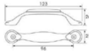
Model: SYJ0247 Material: Zinc & Ceramic Chrome Plated
