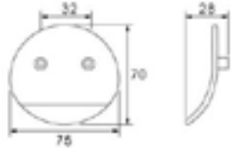
Model: SYJ0136 Material: Zinc Chrome Plated
