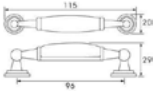
Model: SYJ0244 Material: Zinc & Ceramic Antique Bronze
